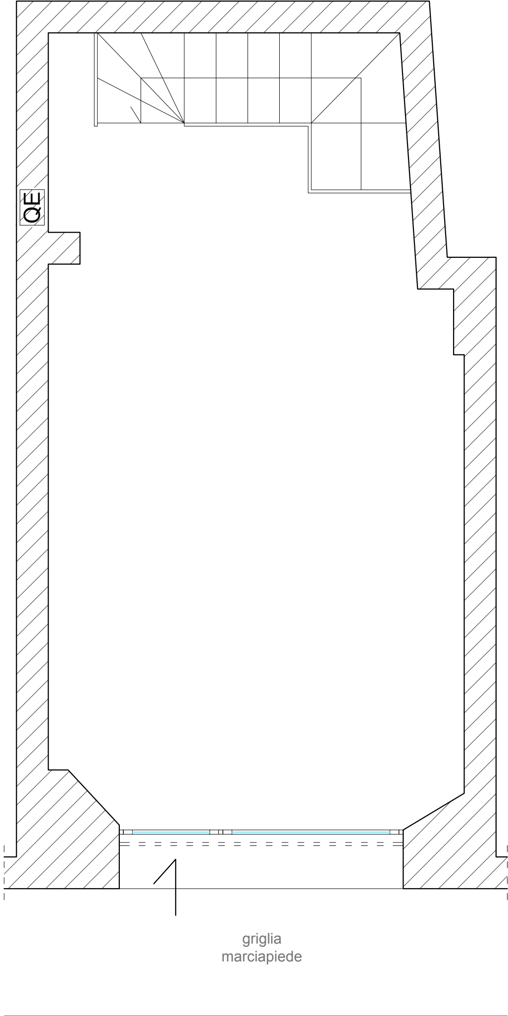
PIANO TERRA
